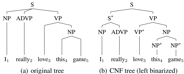
Figure 1: Example constituency trees. Part-of-speech (POS) tags are not used as inputs in this work and thus excluded.
