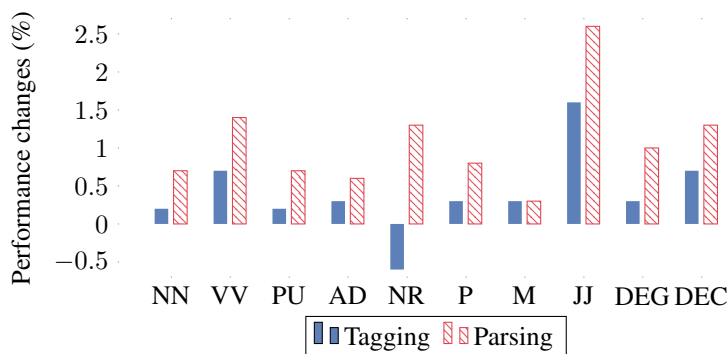
Fig. 3: Changes of tagging accuracy and parsing accuracy (LAS) on the CoNLL09 test set for words of different POS tags. Words/arcs are categorized according to their/their dependent’s gold-standard POS tags.
